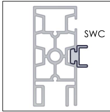
SLOTWALL CHANNEL
